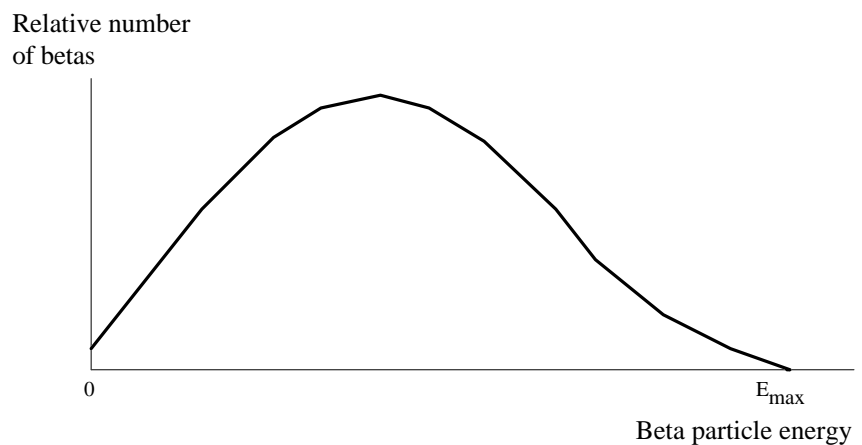
Figure 2.1 Typical Beta Spectrum
